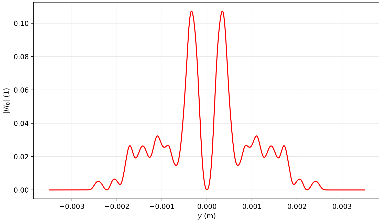
Intensity profile I(x=0, y, z=2.548)/I_0 , P_{in}=8.0P_{cr} , artificial time
